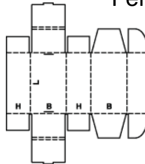
Fefco 0427
